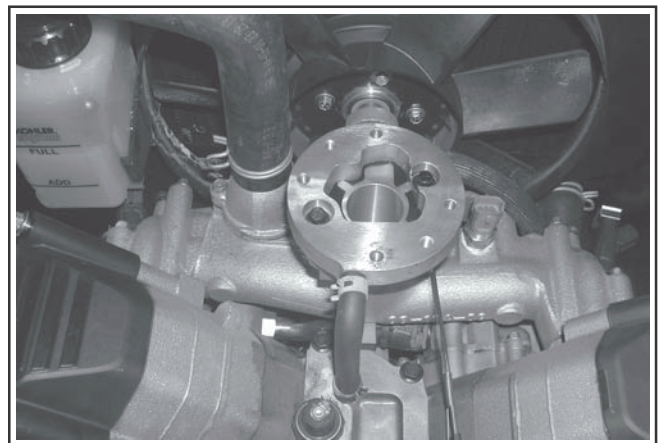
Figure 27. EFI Throttle Body Manifold.
